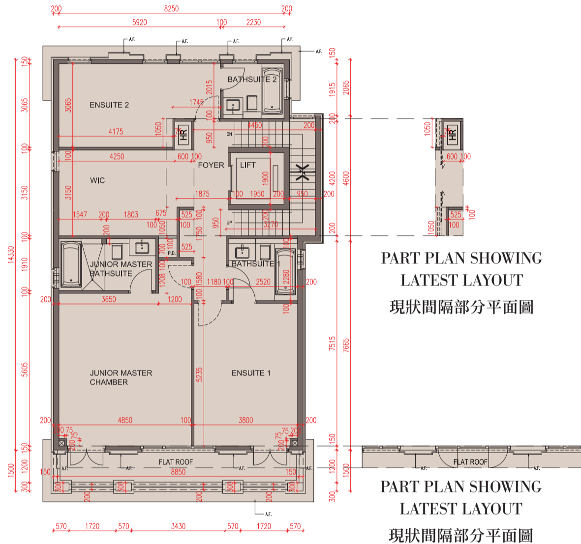
FIRST FLOOR PLAN 一樓平面圖
